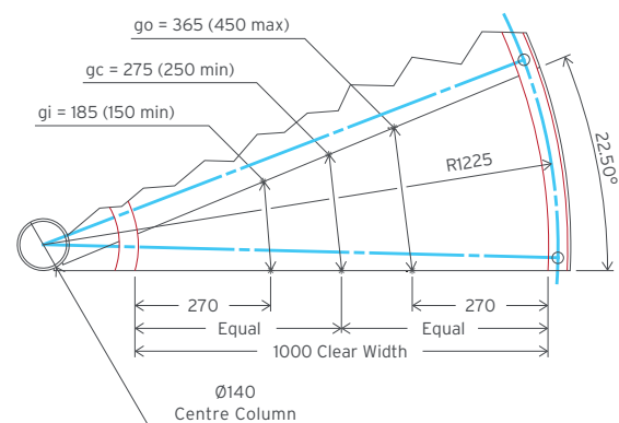
Fig 1. Steel staircase tread geometry (mm) Overall Ø = 2500* / 16 treads per 360° revolution
