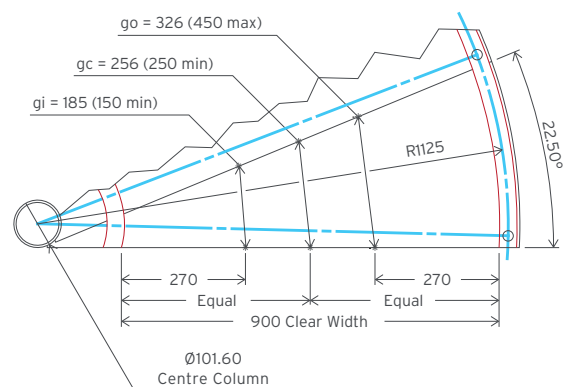
Fig 1. Steel staircase tread geometry (mm)
