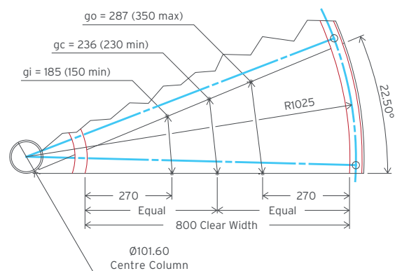
Fig 1. Steel staircase tread geometry (mm) Overall Ø = 2100* / 16 treads per 360° revolution
