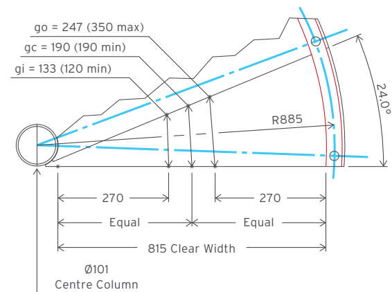
Fig 1. Steel staircase tread geometry (mm) Overall Ø = 1820* / 15 treads per 360° revolution
