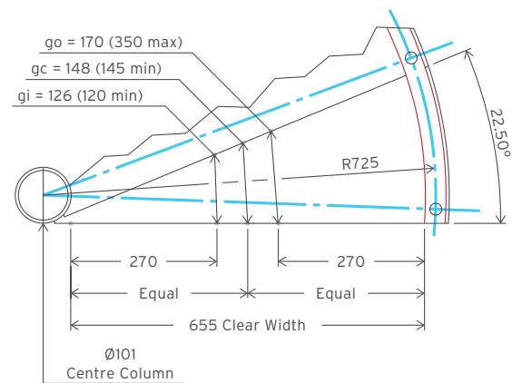
Fig 1. Steel staircase tread geometry (mm) Overall \varnothing = 1500^* / 16 treads per 360^\circ revolution
